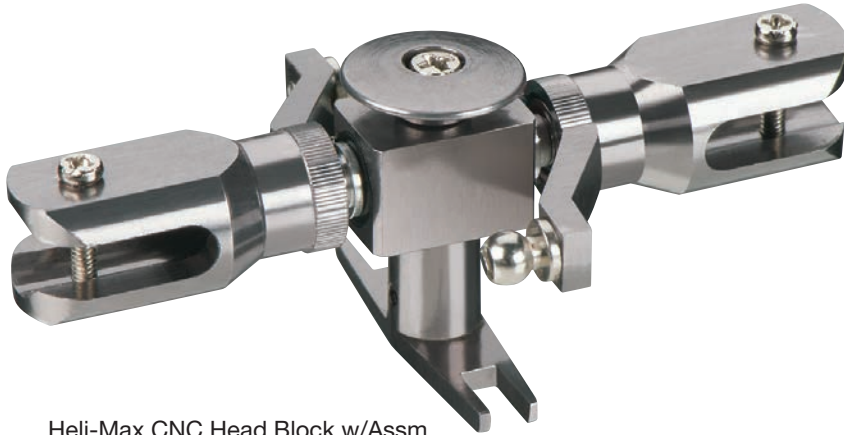
Heli-Max CNC Head Block w/Assm. Blade Grips Axe 100 CP/SS
