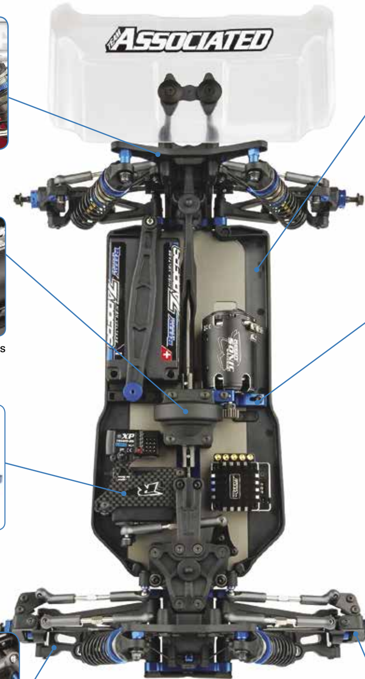
7075 anodized narrow aluminum chassis with lightweight side guards
