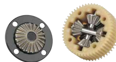
Gear differential More corner speed and forward acceleration
