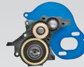
New transmission has stronger gears, precision ball bearings and a 14 carbide ball differential. Transmission shown is for the RC10B5.
