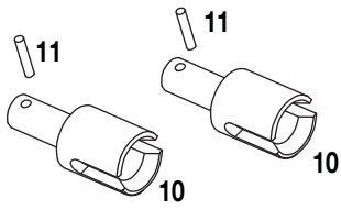
Differential Joint Set DTXC7341
